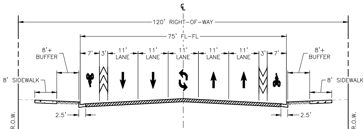
4-LANE MINOR ARTERIAL WITH SEPARATED BIKE LANES (URBAN AND SUBURBAN)
