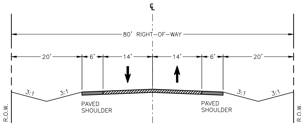
RURAL ARTERIAL 2 LANES
