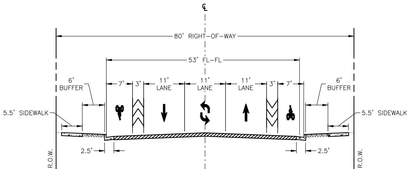
2-LANE COLLECTOR WITH CENTER LEFT TURN LANE AND SEPARATED BIKE LANES (URBAN AND SUBURBAN)
