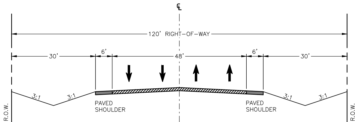
RURAL PRINCIPAL ARTERIAL/RURAL ARTERIAL 4 LANES
