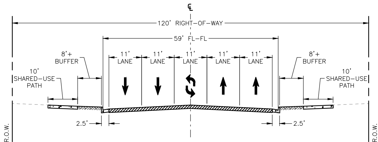
4-LANE MINOR ARTERIAL WITH SHARED-USE PATHS (URBAN AND SUBURBAN)
